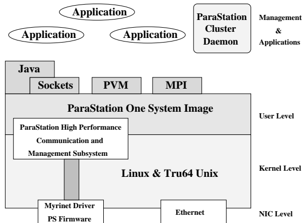
Figure 1: Overview of the ParaStation3 system
